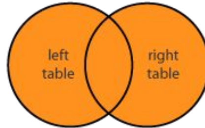
FULL JOIN
