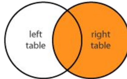
RIGHT JOIN
